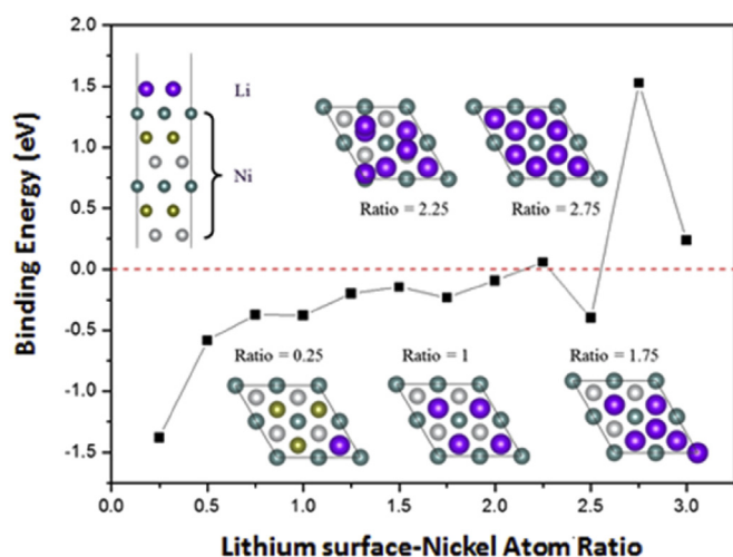
Fig. 5. Binding energy with different lithium surface-nickel atom ratios. The inset figures indicate configurations of different lithium atom numbers. Different nickel atoms are in different colors according to their positions. (For interpretation of the references to color in this figure legend, the reader is referred to the Web version of this article.)
