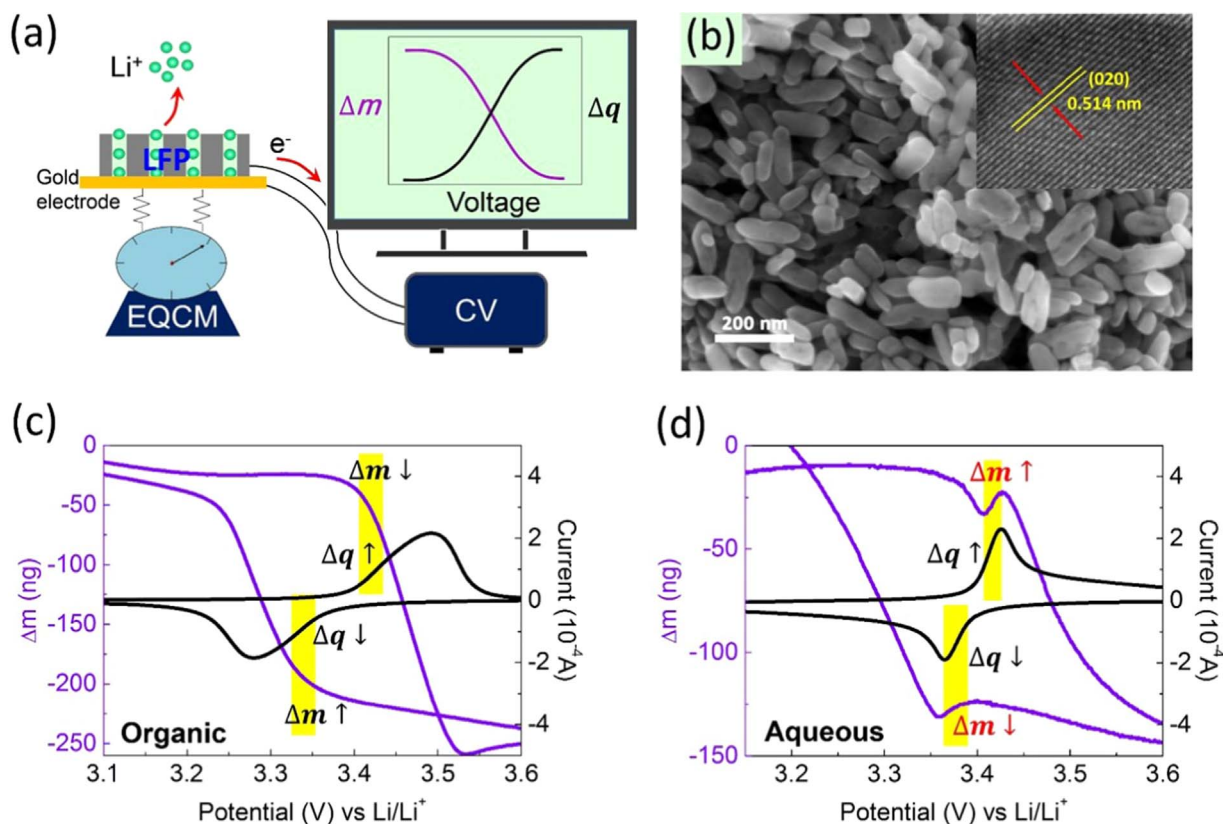
Fig. 1. (a) The schematic of the charging process of \text{LiFePO}_4 electrode in an EQCM apparatus, the picture in the right-top corner illustrates that as the total mass ( M , purple line) of the electrode monotonically decrease as the charge capacity ( Q , black line) increasing. (b) Morphology of the 100 nm particle with the mostly exposed surface detected to be (010). (c) The mass-potential cure (purple line) and CV curve (black line) of \text{LiFePO}_4 in organic electrolyte where the mass decrease (increase) monotonically in the charging (discharging) process, as illustrated in the upper (lower) highlighted area. (d) The mass-potential cure and CV curve of \text{LiFePO}_4 in aqueous electrolyte where the mass increase (decrease) shows an AMCI, which is the highlighted parts of the purple curves, in the charging (discharging) process, as shown in the upper (lower) highlighted area.
