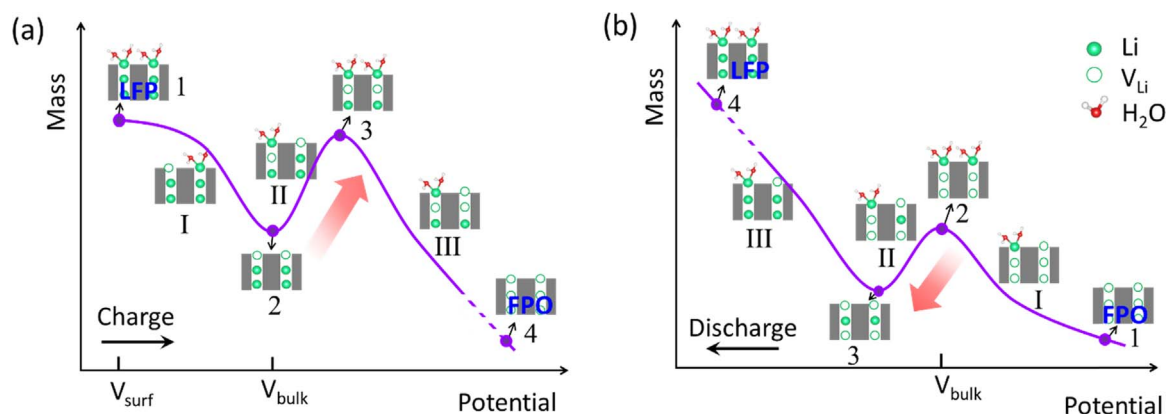
Fig. 6. (a) The simulated mass-potential curve of the charging process for \text{LiFePO}_4 in aqueous system at different stages. The high-lighted stage (II) illustrates that the re-adsorption of water molecule on the (010) surface leads to the abnormally mass increase. (b) The simulated mass-potential curve of the discharging process in aqueous system at different stages. The highlighted stage II illustrates that the re-desorption of water molecule on the (010) surface leads to the abnormally mass decrease.
