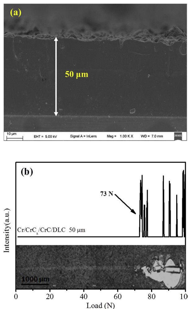
Fig. 9. (a) SEM cross-sectional images and (b) Scratch test of the 50\text{ }\mu\text{m} DLC coating.
