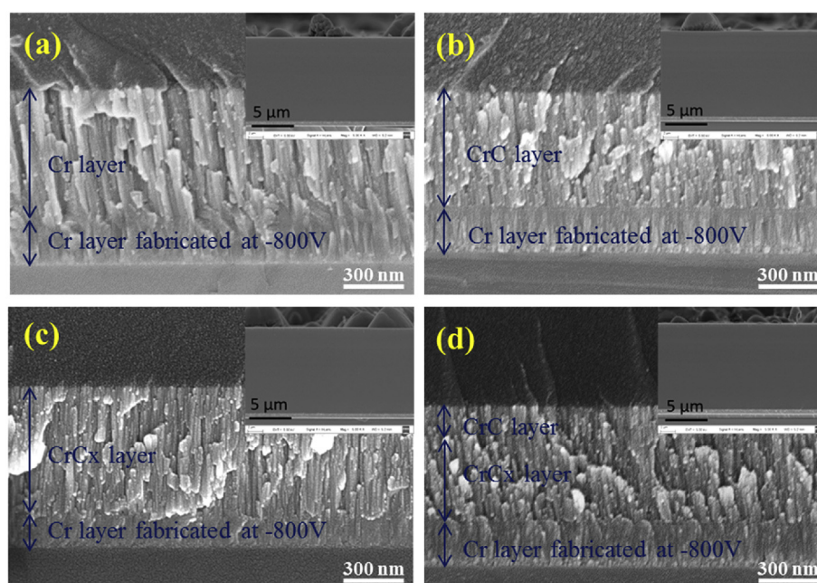
Fig. 2. SEM cross-sectional images: (a) Cr/DLC, (b) Cr/CrC/DLC, (c) Cr/CrCx/DLC, and (d) Cr/CrCx/CrC/DLC.
