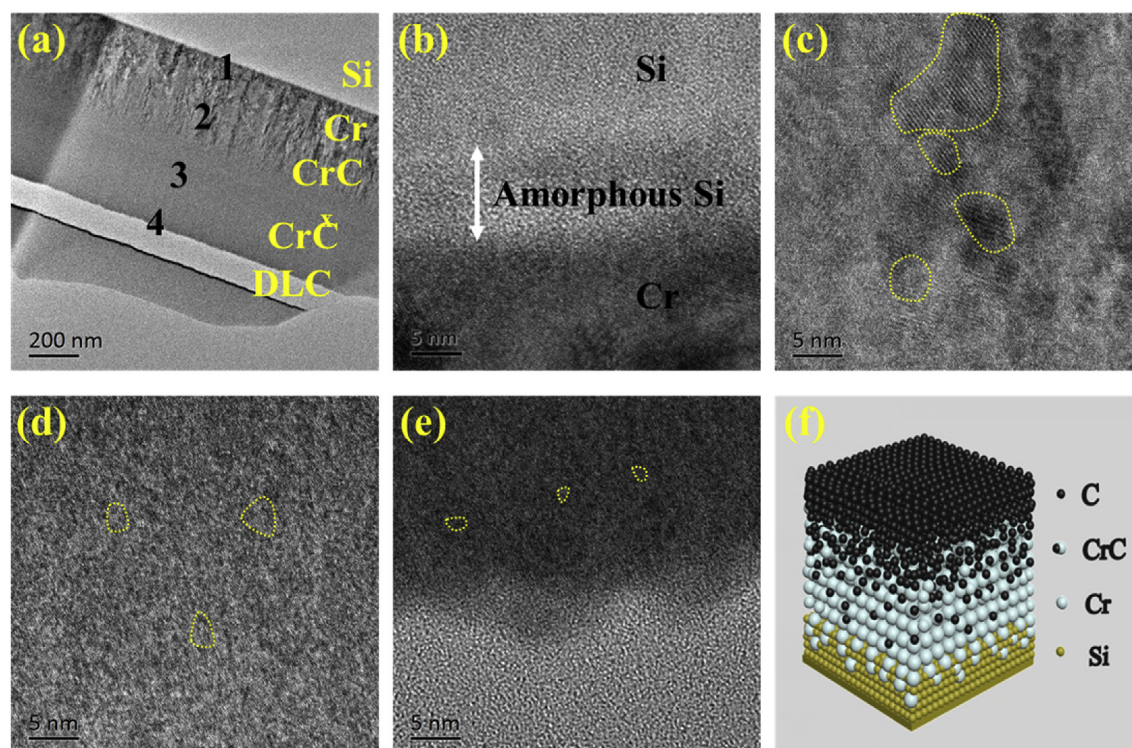
Fig. 10. (a) Cross-sectional image of Cr/CrCx/CrC/DLC; (b–e) High-magnification images of positions 1, 2, 3, and 4; (f) Sketch map of Si/Cr/CrCx/CrC/DLC.
