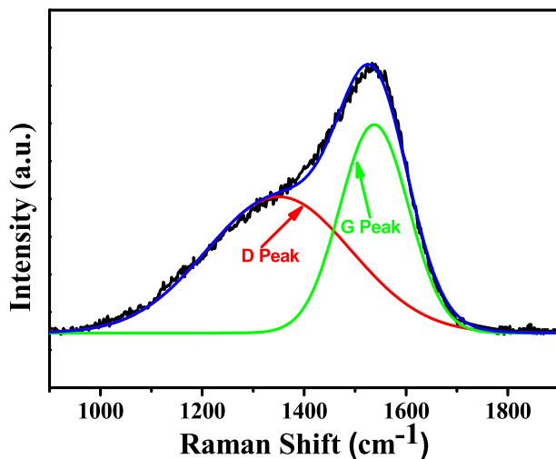
Fig. 4. Representative Raman scattering spectra of Cr/CrCx/CrC/DLC.
