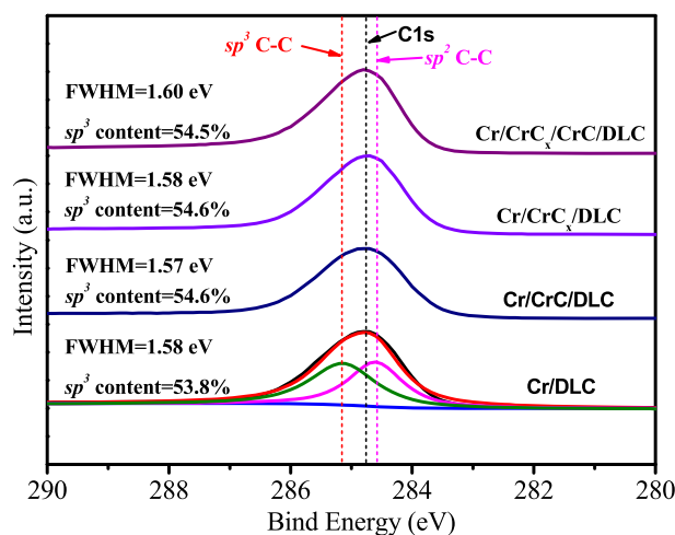
Fig. 5. XPS C1s spectra of the DLC coatings.
