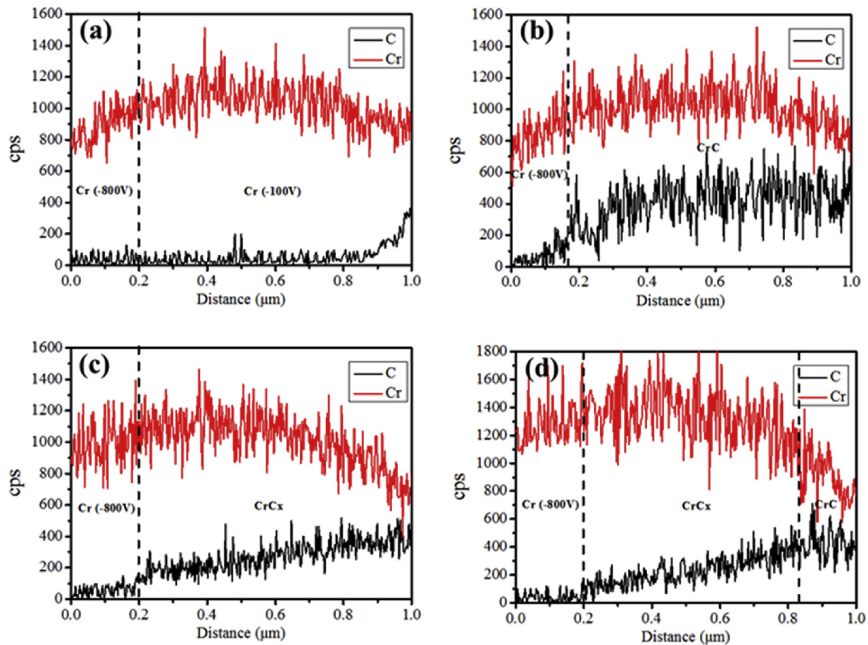
Fig. 3. The C and Cr cross-sectional distribution of different interlayers: (a) Cr, (b) Cr/CrC, (c) Cr/CrCx, and (d) Cr/CrCx/CrC.
