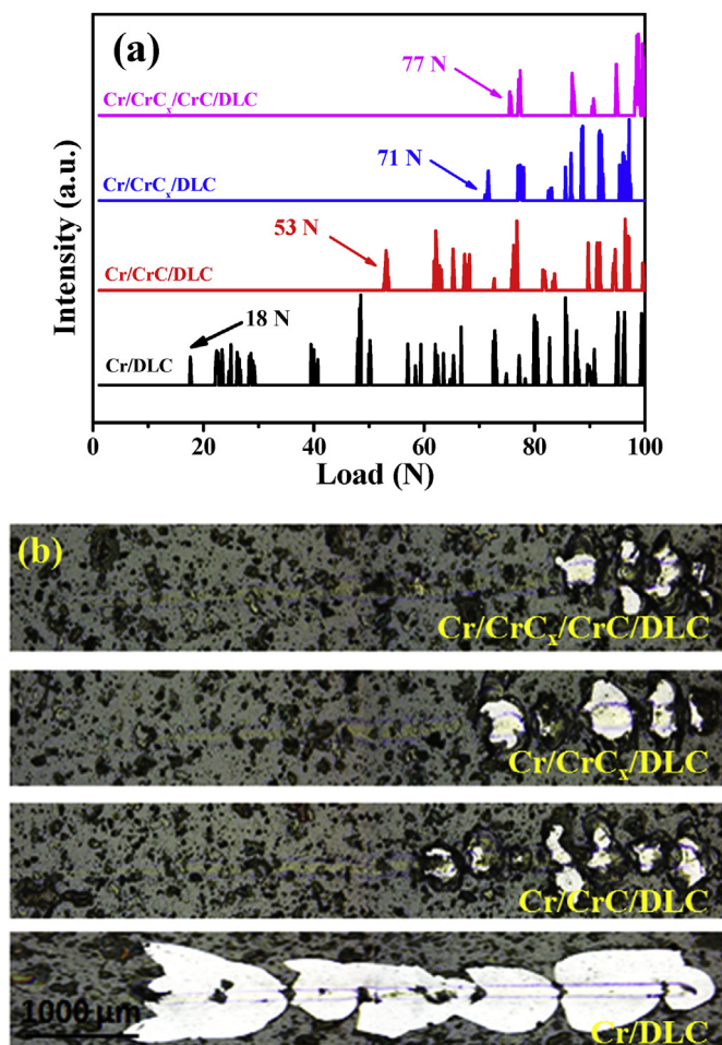
Fig. 8. Scratch test results of the DLC coatings: (a) Acoustic emission signal and (b) Scratch morphology.
