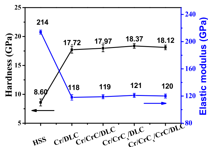
Fig. 6. Hardness and elastic moduli of the HSS and DLC coatings.
