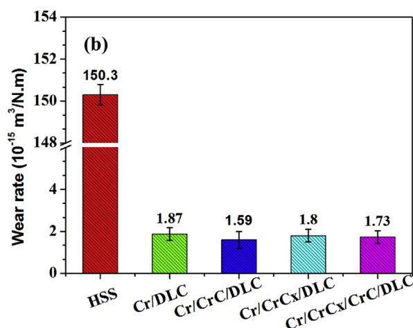
Fig. 7. Friction test of HSS and DLC coatings: (a) Friction coefficients and (b) Wear rates.
