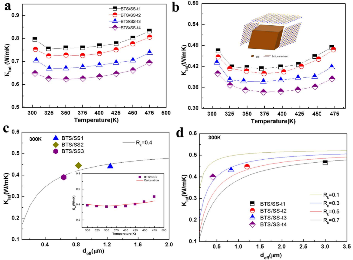
Fig. 4. (a) Temperature dependence of \kappa_{tot} for the BTS/SS nanocomposites with different thickness of SnS 2 nanosheet. (b) lattice thermal conductivity ( \kappa_{latt} ). (c) Room temperature lattice thermal conductivity with varying effective grain size (determined by the content of SnS 2 , the inset is the \kappa_{latt} of BTS/SS3 compared with the calculated results from Eq. (1)). (d) Room temperature lattice thermal conductivity of BTS/SS nanocomposites with different thickness of SnS 2 nanosheet.
