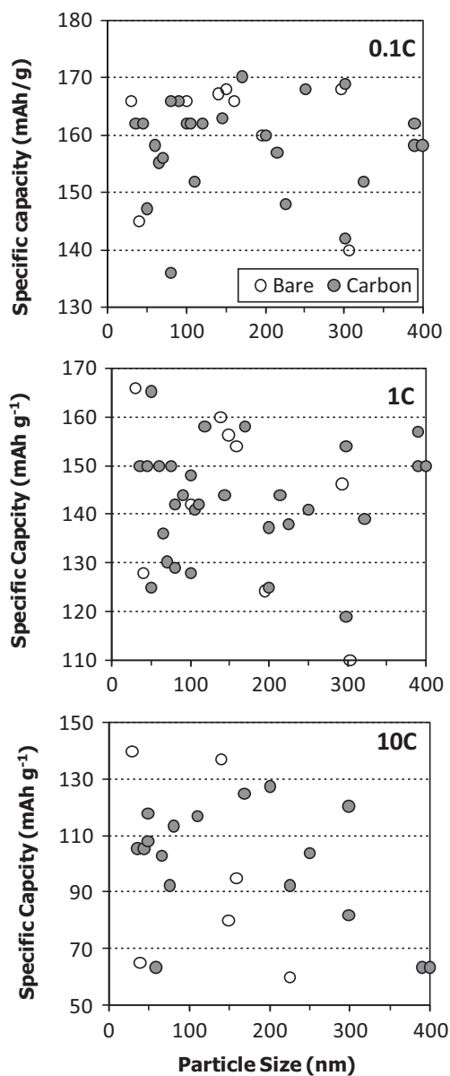
Fig. 5. The dependence of specific capacity at 0.1 C, 1 C and 10 C rates on the particle size of LiFePO 4 with or without carbon coating [45]. Reproduced with permission from The Electrochemical Society.
