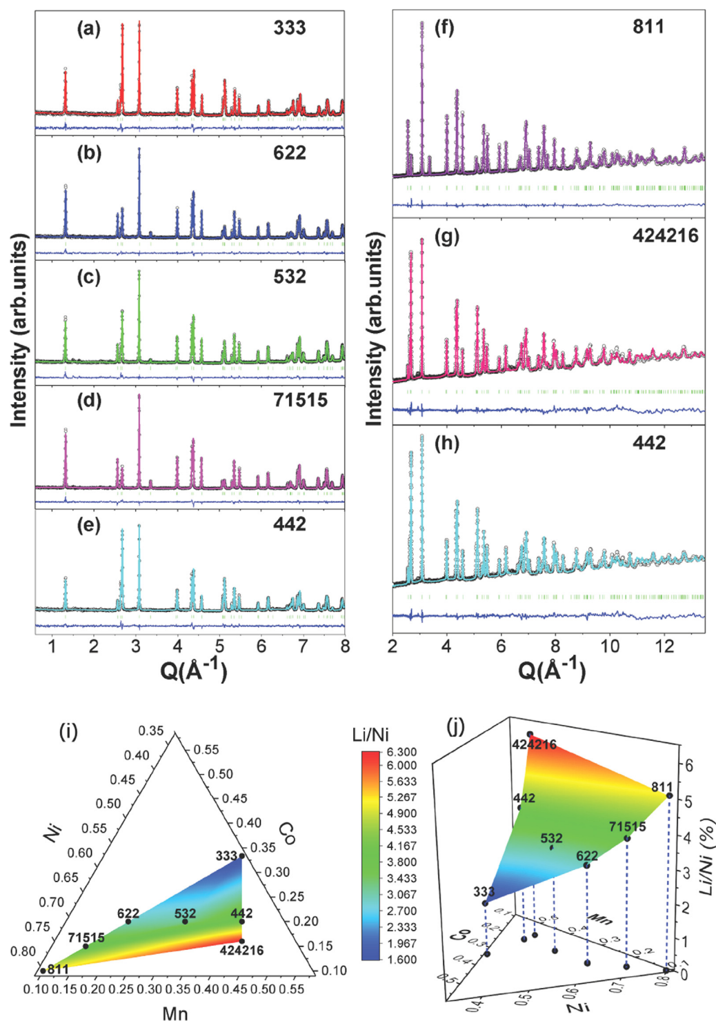
Fig. 4. Neutron powder diffraction refinement patterns for series of \text{Li}_{1-x}\text{Ni}_x\text{Mn}_y\text{Co}_z\text{O}_2 compounds based on the data collected at BT1(a-e) and GPPD(f-h), respectively. (i) and (j) Li/Ni exchange ratios of \text{Li}_{1-x}\text{Ni}_x\text{Mn}_y\text{Co}_z\text{O}_2 compounds with different compositions of transition metals.
