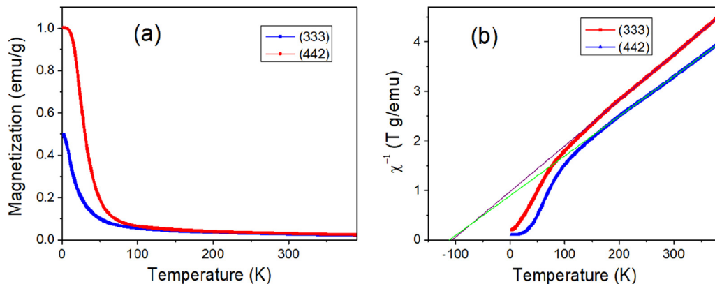
Fig. 3. Temperature dependence of the magnetization (a) and inverse magnetic susceptibility (b) of (333) and (442) measured under magnetic field of 1000 Oe.
