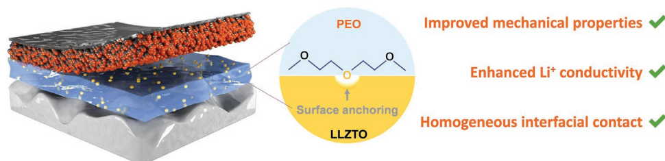
Scheme 1. Proposed working mechanisms for OV-LLZTO/PEO in an all-solid-state battery.
