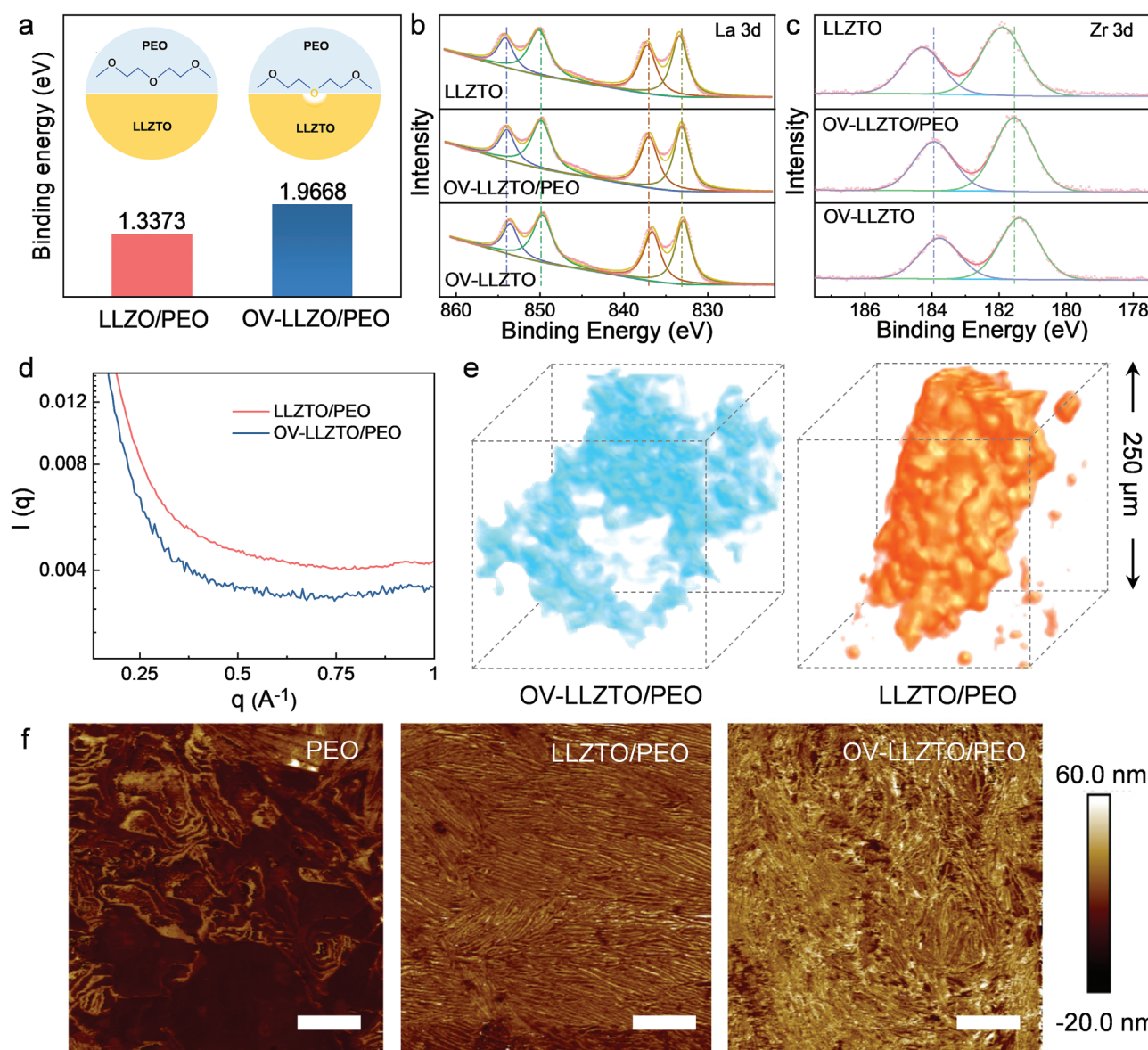
Figure 2. Improved mechanical properties enabled by oxygen vacancies. a) Simulated binding energy between different fillers and PEO. XPS analysis of solid electrolyte membranes: b) La3d spectra and c) Zr3d spectra. For better signal-noise ratios, the weight content of OV-LLZTO in the membrane is 50 wt.%. d) SAXS profiles of solid electrolyte membranes with a filler content of 50 wt.%. e) 3D structures of solid electrolyte membranes with 50 wt.% of fillers from X-ray micro-computed tomography, where the blank, blue and orange regions represent PEO, OV-LLZTO and LLZTO respectively. f) AFM deformation images of different solid electrolytes (scale bar = 2 \mu\text{m} ).
