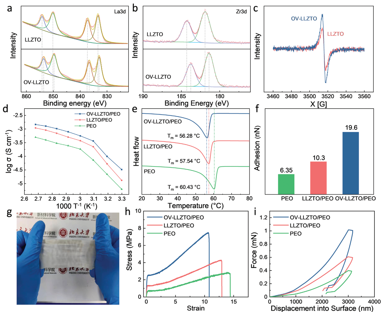
Figure 1. Characterizations of OV-LLZTO/PEO. a) La3d spectra and b) Zr3d spectra. c) EPR spectra of the pristine LLZTO and OV-LLZTO. d) Arrhenius plots of different electrolytes under different temperatures. e) DSC curves and the corresponding melting temperatures. f) The average interfacial adhesion force measured by AFM. g) Images of a sizable OV-LLZTO/PEO membrane being stretched. h) Stress–strain curves and i) nano-indentation curves of different membranes.
