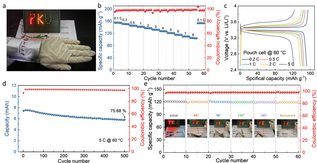
Figure 4. Solid-state pouch cell performance. a) Photograph of the flexible pouch cells. b) Rate performance under different C-rates and c) the corresponding voltage curves. d) Cycling performance under 5 C. e) Demonstration of foldability of the pouch cell (inset photos) and the cycling performance when bent to different angles. All galvanostatic cycling tests are carried out at 60 °C and photos are taken at room temperature.
