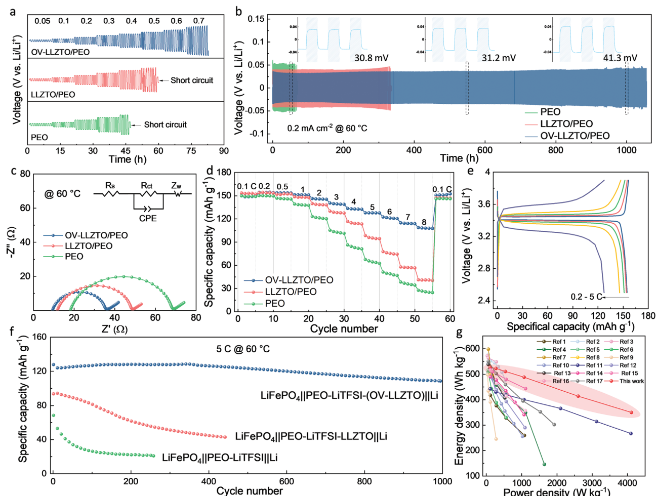
Figure 3. Improved electrochemical performance. a) Stepped current density galvanostatic cycling under different current density, b) galvanostatic cycling curves under 0.2 \text{ mA cm}^{-2} , and c) EIS of Li-Li symmetric cells using different solid electrolytes. d) Rate performance of all-solid-state LFP batteries using different electrolytes and e) corresponding voltage curves of the cell using OV-LLZTO/PEO under different C-rates. f) Cycling performance of all-solid-state LFP batteries using different electrolytes under 5 C. All batteries are tested under 60^\circ\text{C} . g) Comparison of the energy and power density with previously reported literatures. The corresponding literatures are listed in Table S4 (Supporting Information).
